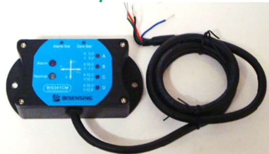
Tilt switch X & Y, 2 axis, 4 fixed alarm settings 5° & 5°, 7.5° & 10°, 12.5° & 10°, 12.5° & 15°, 2 sec delay, easy 0° set, (0.8m lead), fail safe, beeps on start up after 5 sec for 1 sec, 2 amp, programable if required, full EWP safety compliant – EMSBIS341CM (This is what we are using in from mid 2025)
