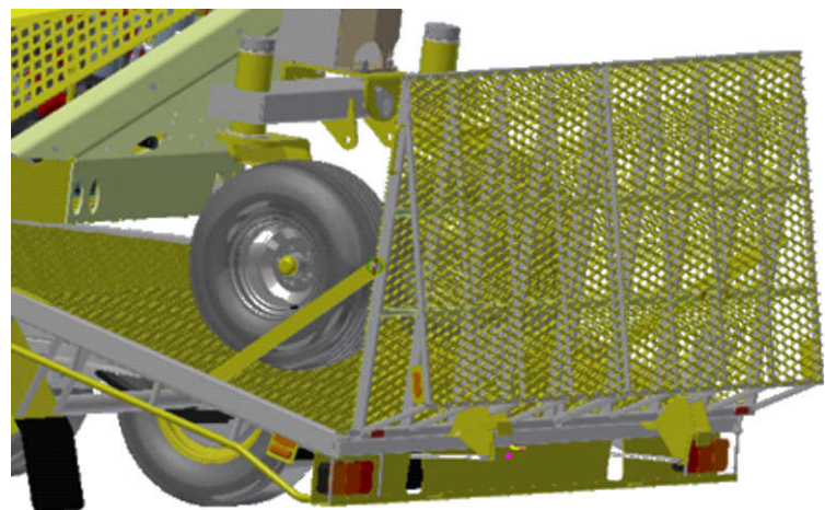
Ramps held up with 2 x side braces clipped on. Four gas struts make this easy to swing up
