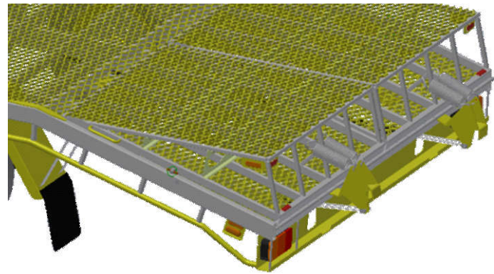
Ramps folded right over to give flat top. Four tension springs make this easy to swing over
